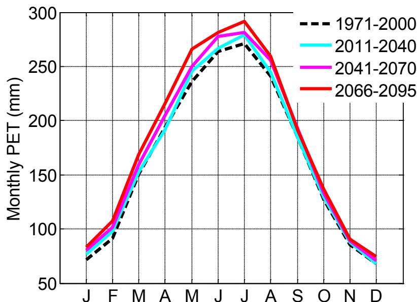
FIGURE C15-9 Monthly Changes in Simulated PET Under three future conditions compared to historical climate.
