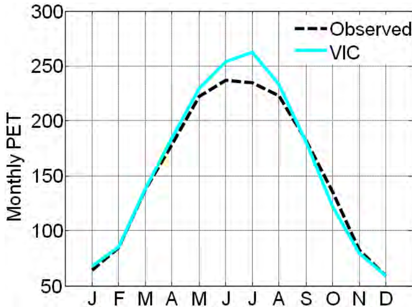
FIGURE C15-1 Comparison of Observed PET and Simulated PET for the Calipatria/Mulberry Station (CIMIS station #41) in California's Imperial Valley
